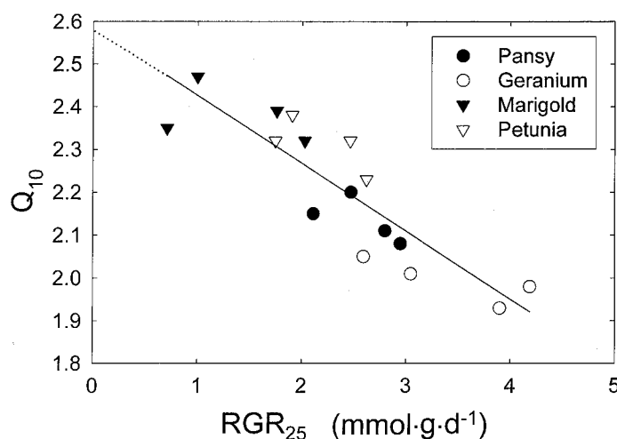
Fig. 5. The correlation between the Q_{10} for dark respiration and the estimated relative growth rate at 25 °C, assuming a 12-h photoperiod. Data from all four species were combined for the regression analysis ( Q_{10} = 2.58 - 0.16 \times RGR_{25} , r = -0.87 ). The Q_{10} for maintenance respiration can be estimated from the Y-intercept of the regression line, because there is no growth respiration when the relative growth rate (and thus growth) is zero.
