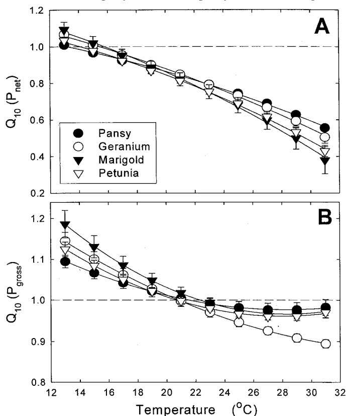
Fig. 2. The Q_{10} of A) net photosynthesis ( P_{\text{net}} ) and B) gross photosynthesis ( P_{\text{gross}} ) of four bedding plant species at different air temperatures. Data points are the mean \pm 1 standard error ( n = 4 ). Error bars not shown are within the limit of the symbol.
