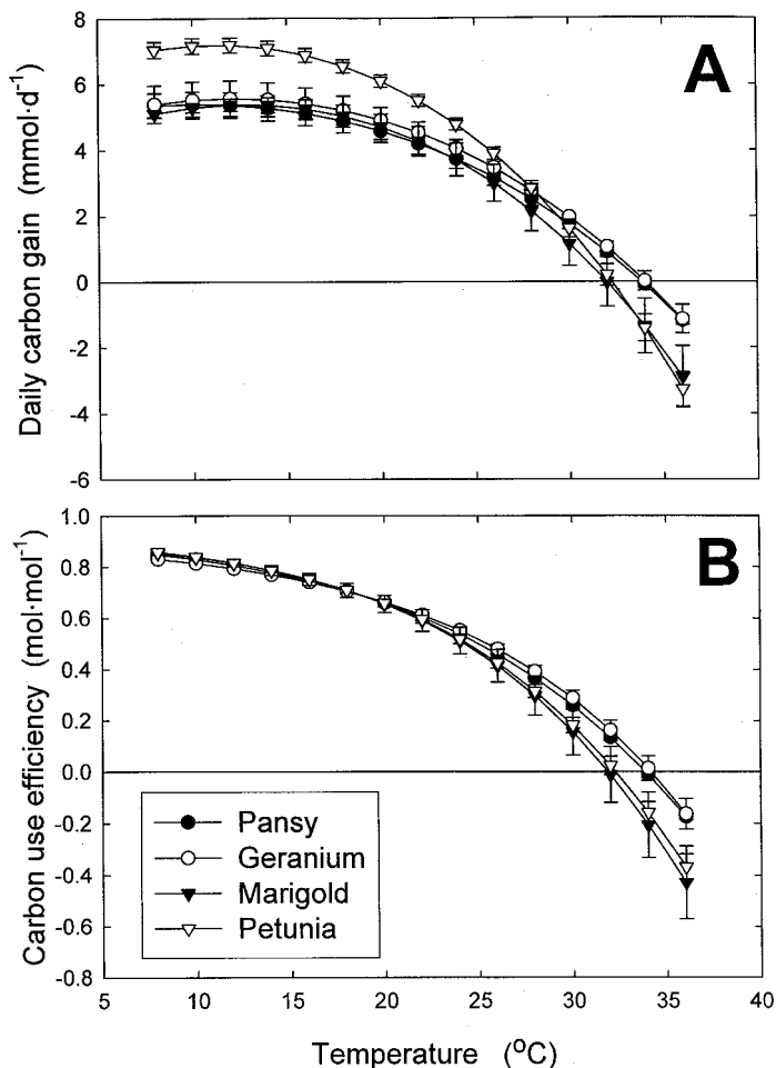
Fig. 3. The effect of short-term changes in air temperature on (A) the daily carbon gain (DCG), a measure of plant growth rate, and (B) carbon use efficiency (CUE), the ratio of carbon incorporated into the plant to the amount of carbon fixed in gross photosynthesis, of four bedding plant species. Data points are the mean (per plant) \pm 1 standard error ( n = 4 ). Error bars not shown are within the limit of the symbol.
