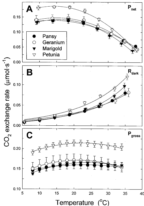
Fig. 1. Air temperature effects on the CO 2 exchange rate of four bedding plant species. (A) Net photosynthesis ( P_{\text{net}} ) was measured at eight different temperatures during a 24 h period (3 h per temperature, increasing from 8 to 38 °C). (B) Dark respiration ( R_{\text{dark}} ) was measured during the subsequent 24 h, with temperatures decreasing from 36 to 6 °C. (C) Gross photosynthesis ( P_{\text{gross}} ) was estimated as the sum of the regression curves fitted to the P_{\text{net}} and R_{\text{dark}} data. Net photosynthesis data were fitted with a quadratic model ( R^2 > 0.98 ), and R_{\text{dark}} data with an exponential model ( R^2 > 0.97 ). Data points are the mean gas exchange rates per plant \pm 1 standard error ( n = 4 ). Error bars not shown are within the limit of the symbol.
