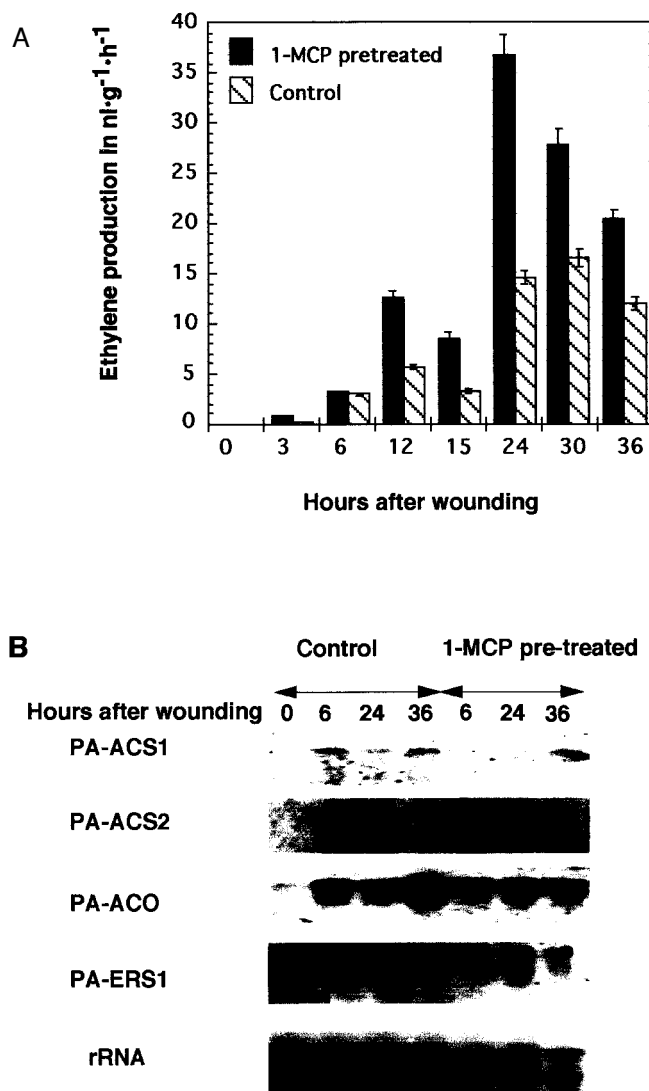
Fig. 4. Time course analysis of wound induced ethylene biosynthesis. (A) Comparison of the ethylene production rates of wounded tissue after 1-MCP pretreatment or without 1-MCP pretreatment. Preclimacteric avocados were either held in air (control) or in the presence of 1-MCP at 20 °C for 24 h and subjected to wounding by slicing into small pieces. Ethylene production was determined at the times indicated. Data are mean values of three replications \pm SE. (B) The effect of 1-MCP pretreatment on PA-ACS1 , PA-ACS2 , PA-ACO and PA-ERS1 transcripts abundance after wounding. After determination of ethylene production at 0, 6, 24, and 36 h time points in A, samples were withdrawn and immediately frozen in liquid \text{N}_2 for subsequent Northern analysis. Details of the Northern blot are as described in the legend of Fig. 3.
