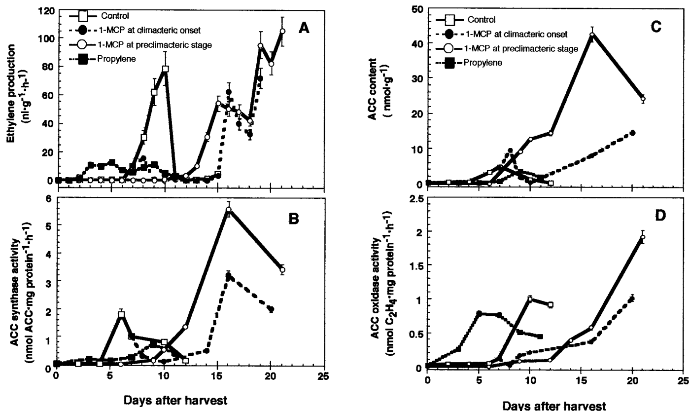
Fig. 2. Changes in ethylene production rate (A), ACC synthase activity (B), ACC content (C), and in vitro ACC oxidase activity (D) during ripening of avocados and the effect of 1-MCP or propylene applied for 24 h at 20 °C. Fruit harvested were either ripened naturally or subjected to 5 \mu\text{L} \cdot \text{L}^{-1} 1-MCP treatment after harvest or at the climacteric rise or to propylene treatment at a concentration of 5000 \mu\text{L} \cdot \text{L}^{-1} . Results are mean values of 10 fruit \pm SE in A and three replications \pm SE in B, C, and D.
