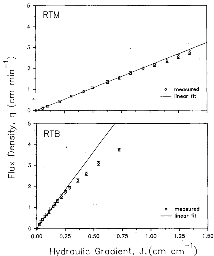
Fig. 6. Flux density vs. hydraulic gradient. The linear range indicates the range of validity of Darcy's law over which the value of K_s was determined.
