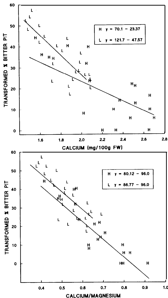
Fig. 2. Relationships between \bar{Ca} concentration (top) or \bar{Ca} : \bar{Mg} ratios (bottom) and bitter pit incidence. Data for heavy-(H) and light-(L) cropping trees are the individual values for six size classes from four orchards. Bitter pit values are arcsin transformations. Lines were fitted as described in Results.
