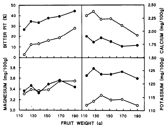
Fig. 1. Bitter pit incidence and Ca, Mg, and K concentrations of fruit from heavy-(●) and light-(○) cropping trees. Data are the means from four orchards for each fruit weight. SEDs and P values for the mean data are given in Table 1.
