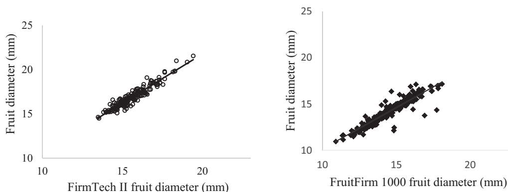
Fig. 2. Linear relationship of 'Legacy' northern highbush blueberry ( Vaccinium corymbosum ) fruit diameter measured by hand and by two firmness-testing machines: FirmTech II (Bioworks Inc., Wamego, KS, USA) and FruitFirm 1000 (CVM Inc., Pleasanton, CA, USA). For FirmTech II, the linear equation is y = 1.9 + 0.811x ( R^2 = 0.903 ); for FruitFirm 1000, the linear equation is y = 1.2 + 0.893x ( R^2 = 0.850 ); 1 mm = 0.0394 inch.
