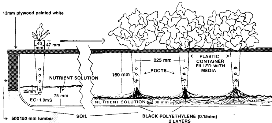
Fig. 1. A capillary, noncirculating hydroponic method for leaf and semi-head lettuce.
