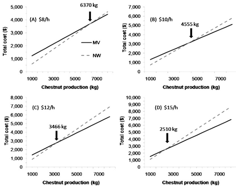
Fig. 2. Sensitivity analysis of total costs (equipment and labor costs) for a modified pasture vacuum [Maxi Vac (MV); Greystone Vacuums, Monroe, WA] and a manual nut-harvesting tool [Nut Wizard (NW); Holt's Nut Wizard, Douglas, GA] at various chinese chestnut production levels and wage rates of (A) $8 per hour, (B) $10 per hour, (C) $12 per hour, and (D) $15 per hour. Values above arrows indicate the production level where total costs of both types of equipment are equal; 1 kg = 2.2046 lb.
