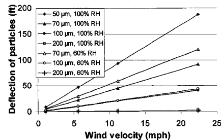
Fig. 1. Effect of windspeed on spray droplet deflection. Droplets discharged at 44 miles/h (mph) ( 20 \text{m}\cdot\text{s}^{-1} ) at a target 1.6 ft ( 0.5 m) below at 68 ^{\circ}\text{F} ( 20 ^{\circ}\text{C} ). RH = relative humidity, 1 ft = 0.3 m, 1 mph = 0.45 \text{m}\cdot\text{s}^{-1} . Adapted from Zhu et al. (1994).
