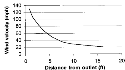
Fig. 2. Effect of distance from outlet on air velocity from a fan jet; 1 ft = 0.3 m, 1 mph = 0.45 m·s -1 . Adapted from Fox et al. (1983).
