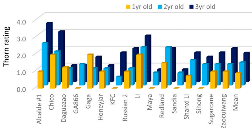
Fig. 3. Thorn lengths on branches of different ages of different jujube cultivars at Alcalde, NM. Evaluation criteria: 0, no thorns; 1, thorns 0 to 6 mm; 2, thorns 6 to 13 mm; 3, thorns, 13 to 25 mm; and 4, thorns >25 mm. KFC, 'Kongfucui'.
