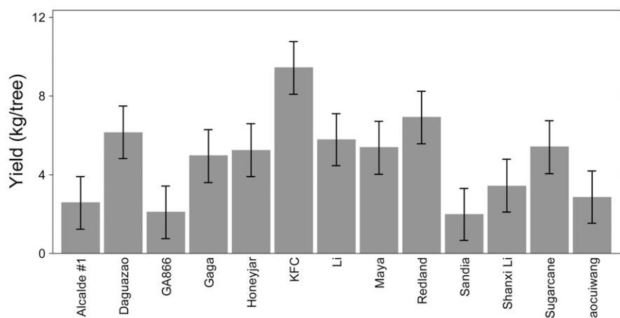
Fig. 1. Average yields of 13 fresh eating jujube cultivars at both Alcalde and Los Lunas across 2017 and 2018. The bars are 95% confidence interval error bars and if they do not overlay, the different between two means are significant at P \leq 0.05 . KFC, 'Kongfucui'.
