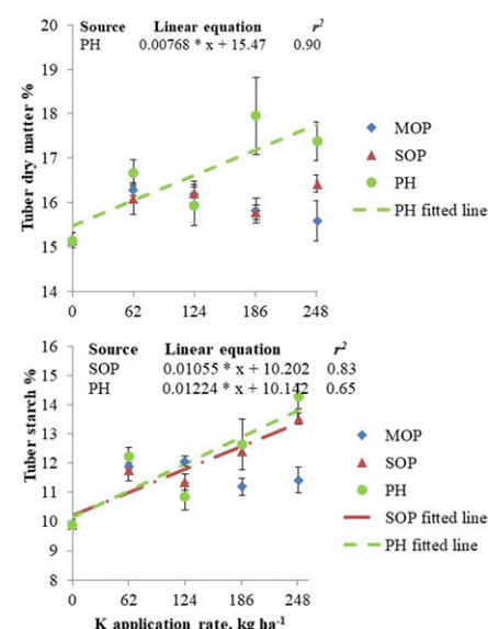
Fig. 2. Dry matter content and starch in potatoes for three fertilizer sources over a range of potassium (K) fertilizer application rates at Tapira, Brazil. Error bars indicate standard error of the means. MOP = muriate of potash; SOP = sulfate of potash; PH = polyhalite.
