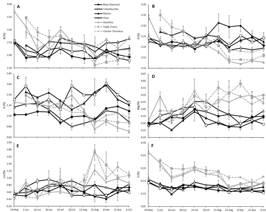
Fig. 1. The effect of sample date over the growing season on the concentration of macronutrients in primocane leaves of floricanefruiting, trailing ('Black Diamond', 'Columbia Star', 'Marion', and 'Onyx'), erect ('Ouachita'), and semierect ('Chester Thornless' and 'Triple Crown') blackberry at the North Willamette Research and Extension Center, Aurora, OR, 2014. A = nitrogen; B = phosphorus; C = potassium; D = magnesium; E = calcium; F = sulfur. Bars indicate standard error for cultivar.
