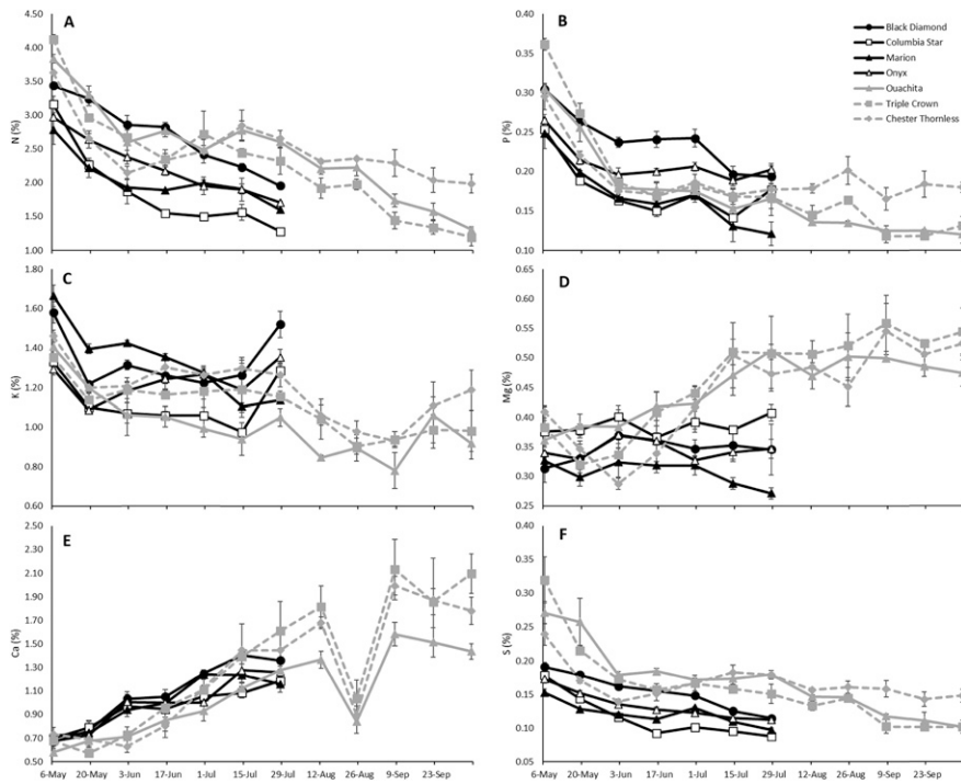
Fig. 3. The effect of sample date over the growing season on the concentration of macronutrients in floricane leaves of trailing ('Black Diamond', 'Columbia Star', 'Marion', and 'Onyx'), erect ('Ouachita'), and semierect ('Chester Thornless' and 'Triple Crown') blackberry at the North Willamette Research and Extension Center, Aurora, OR, 2014. A = nitrogen; B = phosphorus; C = potassium; D = magnesium; E = calcium; F = sulfur. Bars indicate standard error for cultivar.
