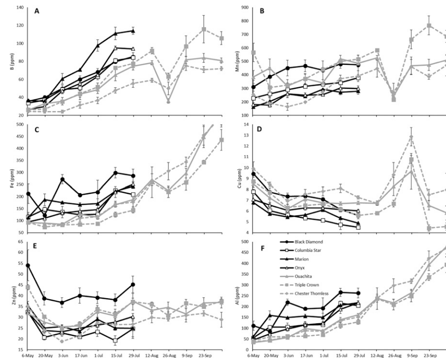
Fig. 4. The effect of sample date over the growing season on the concentration of micronutrients in floricane leaves of floricane-fruiting, trailing ('Black Diamond', 'Columbia Star', 'Marion', and 'Onyx'), erect ('Ouachita'), and semierect ('Chester Thornless' and 'Triple Crown') blackberry at the North Willamette Research and Extension Center, Aurora, OR, 2014. A = boron; B = manganese; C = iron; D = copper; E = zinc; F = aluminum. Bars indicate standard error for cultivar.
