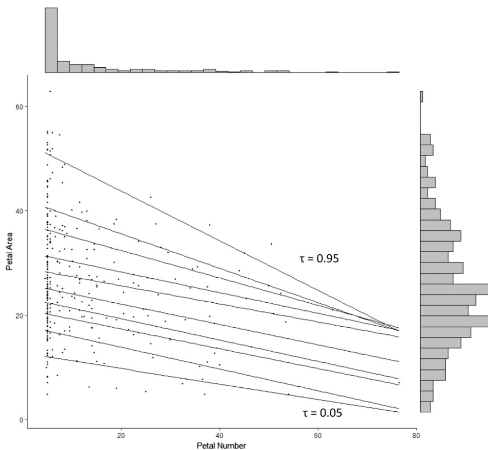
Fig. 1. Petal area and petal number plotted with fitted quantile regression lines (from τ = 0.05 to τ = 0.95) for the simple linear model, Y \sim \beta_0 + \beta_1 X + \varepsilon , and the distributions of the petal area (right) and petal number (upper) among 294 BC 1 F 1 progeny from crosses between several Hibiscus syriacus cultivars and two interspecific hybrids Lohengrin and Resi.
