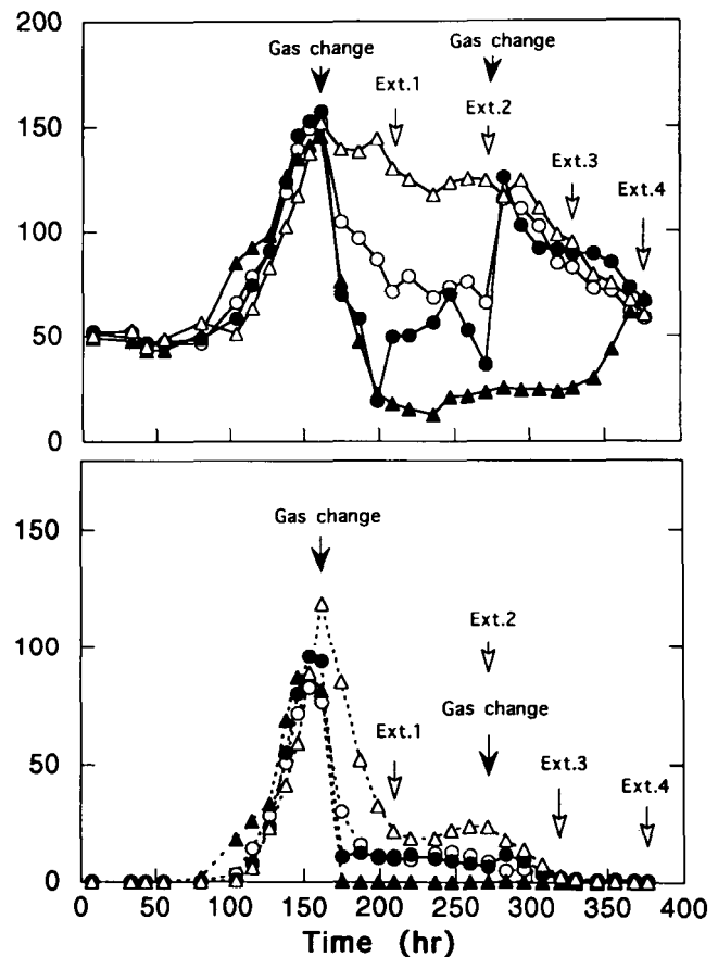
Fig. 1. Respiration (upper graph) and ethylene production (lower graph) by avocados subjected to stress atmospheres at or near the climacteric peak (first closed arrow) and returned to air 105 h later (second closed arrow). Air (A), 25% CO 2 (O), 75% CO 2 (●), N 2 (▲). Mitochondria were extracted from representative fruit at four progressive stages (open arrows) 43 and 105 h after exposure to stress atmospheres and 58 and 105 h after the return to air.
