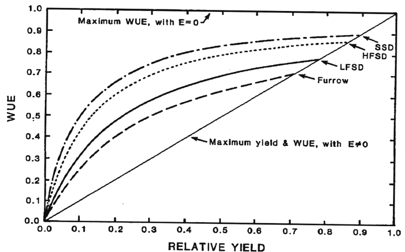
Fig. 2. Effect of irrigation systems and frequencies on water-use efficiency (WUE) of tomatoes (after Phene, 1987). The straight diagonal line represents the maximum relative yields ( j ) and WUE when the ratio (E + T)/(E_p + T_p) = 1 . The curvilinear functions represent the relationships for the four irrigation systems shown in Fig. 1. The horizontal line at the top represents the case where E = 0 and the absolute potential case for all systems under present cultivars and climatic and atmospheric conditions.
