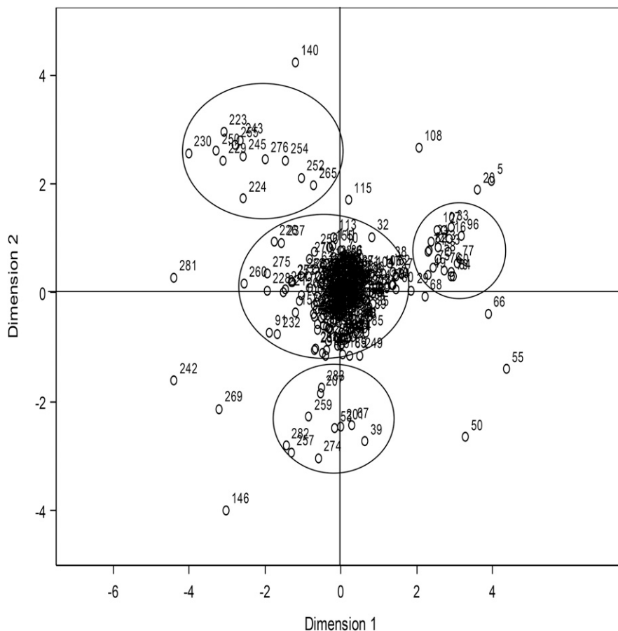
Fig. 4. Plot of the first and second dimension of the multidimensional scaling analysis of genetic relationships among the progeny and parents of the ‘New Kawogo’ (NK) × ‘Beauregard’ (B) sweetpotato mapping population.
