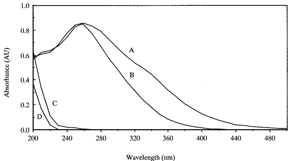
Fig. 2. Absorbance by 89.5 \mu\text{mol}\cdot\text{L}^{-1} solutions of FeDTPA [(A) nonirradiated and (C) irradiated (supernatant)] and FeEDTA [(B) nonirradiated and (D) irradiated (supernatant)]. Solutions were irradiated with 500 \mu\text{mol}\cdot\text{m}^{-2}\cdot\text{s}^{-1} from a fluorescent plus incandescent light source. Soluble Fe concentration in the supernatant of the irradiated solutions was 0. Maximal absorbance by FeDTPA and FeEDTA was 260 and 258 nm, respectively.
